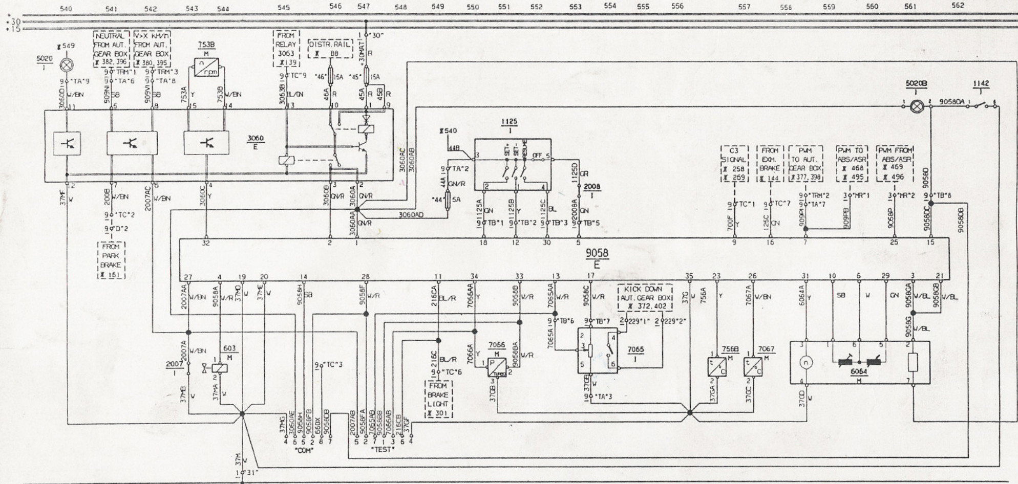
ELECTRONIC DIESEL CONTROL (EDC)
